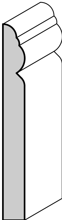
B-395 Base 5/8" X 3-1/4"
