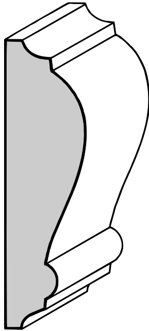
MM-2 Mantel Mould 1" X 3-7/8"
