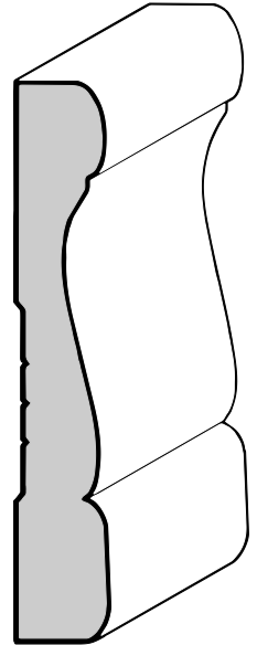
3-1/2" Colonial Casing (C-13) 5/8" X 3-1/2"
