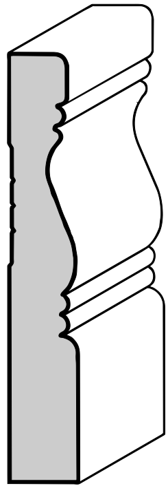
Beaded Colonial Base (B-1) 11/16" X 4-1/4"
