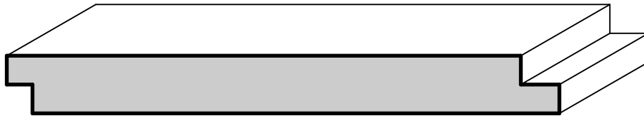
1 X 6 Nickel Gap 9/16" X 5-3/8"
