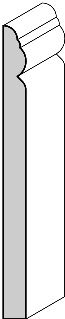
B-695 Base 9/16" X 6-1/2"
