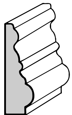
RH Panel Mould 11/16" X 2-1/8"
