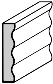
Fluted Batten Strip 1/4" X 1-5/16"
