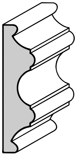
Double PM-7 Chair Rail 11/16" X 2-7/8"
