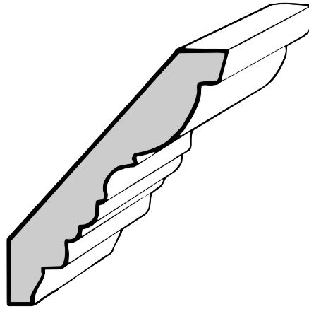
BB-20 Crown 9/16" X 3-1/4"
