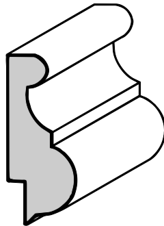
PM-2 w/1/4" Plow 11/16" X 1-5/8"
