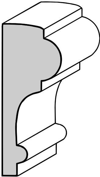
CR-6 Chair Rail 1-3/8" X 3-3/8"
