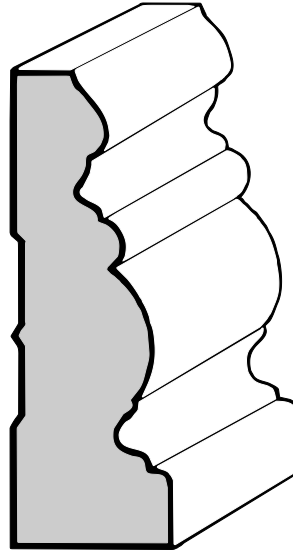
C-422 Casing 1-1/8" X 3-1/2"
