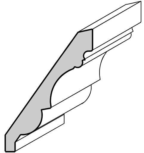
6350 Crown 9/16" X 3-1/2"
