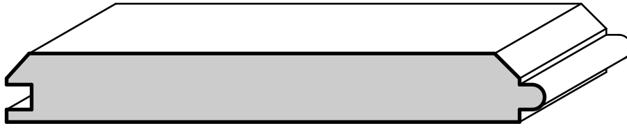
1 X 6 #122 T&G Siding 11/16" X 5-3/8"
