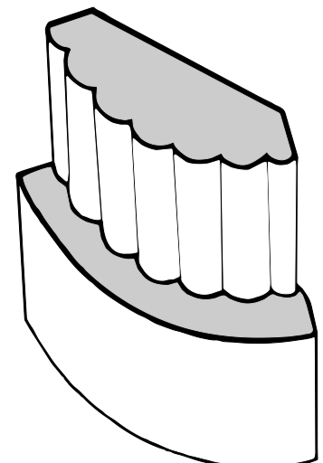
90 Degree Corner Mould 3/4" X 2-1/8" Base 1" X 2-5/8"
