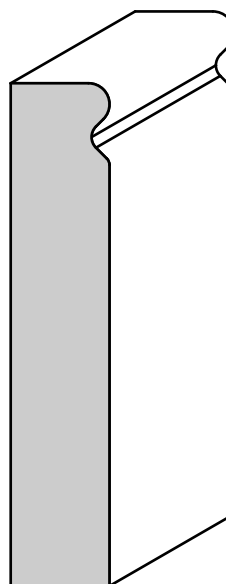
Large PC-1 Casing 11/16" X 3-1/2"
