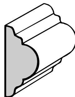
DM-8 Door Mould 3/4" X 1-1/2"
