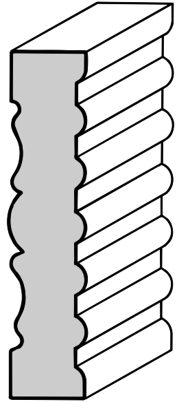
C-14 Casing Reversed 11/16" X 3-1/2"
