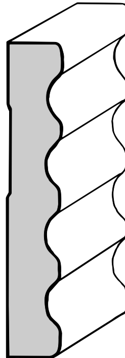
4-1/4" Fluted Casing (C-41) 11/16" X 4-1/4"
