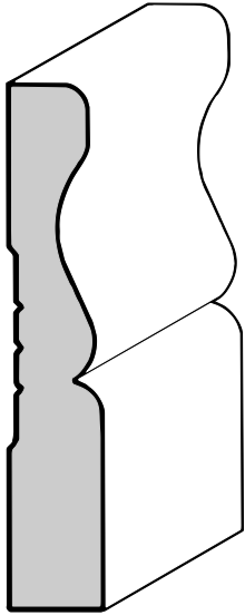
3-1/4" Colonial Base 9/16" X 3-1/4"
