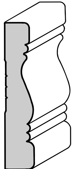
Beaded Colonial Casing (C-1) 11/16" X 3-1/2"
