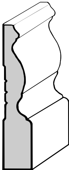
B-322 Base 5/8" X 3-1/4"
