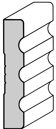
3-1/4" Fluted Casing (C-10) 9/16" X 3-1/4"
