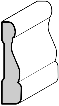
2" Colonial Casing 5/8" X 2"
