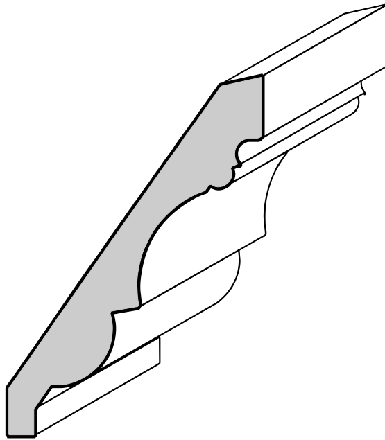
6450 Crown 9/16" X 4-1/2"
