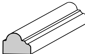
CM-2 3/8" X 1/2"
