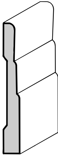
3 Step Base 3/8" X 3"
