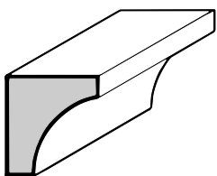
8060 Scotia 3/4" X 7/8"
