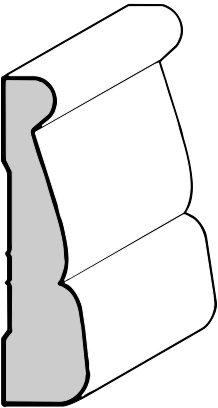
Old Style Colonial Casing 9/16" X 2-3/16"
