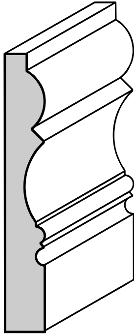
B-3325 Base 11/16" X 4-1/4"
