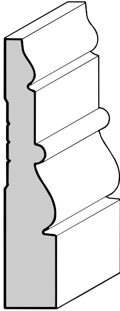
B-3011 Base 11/16" X 3-5/8"
