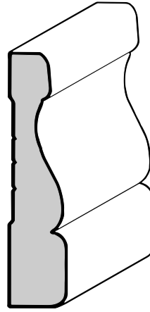
2-1/2" Colonial Casing 9/16" X 2-1/2"
