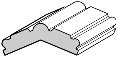
22-1/2 Degree Beaded Outside Corner 3/4" X 1-7/8"
