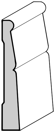
Old Style Colonial Base 7/16" X 3"
