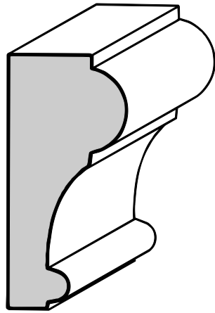
CR-7 Chair Rail 1-1/8" X 2-7/8"
