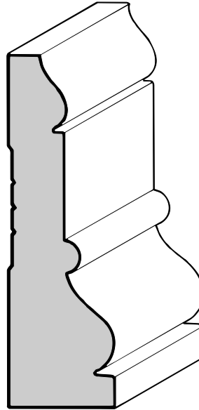
C-11 Casing 1-1/8" X 3-1/2"
