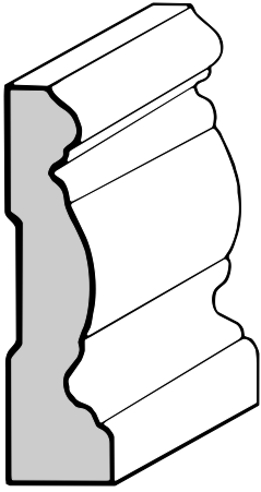
C-322 Casing 9/16" X 2-1/2"
