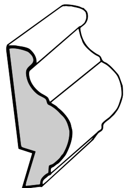
PM-10 3/4" X 2"
