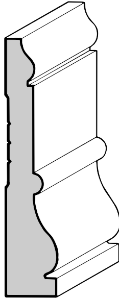
C-3511 Casing 11/16" X 3-1/2"
