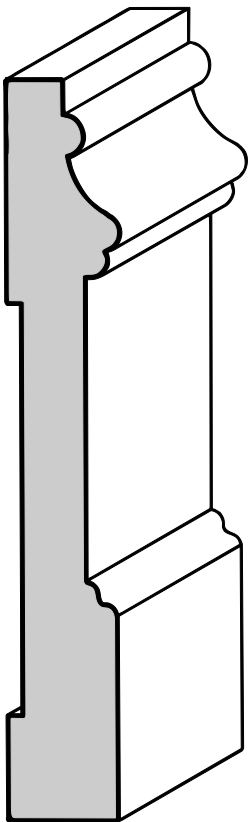
C-16 Casing 11/16" X 5-1/4"
