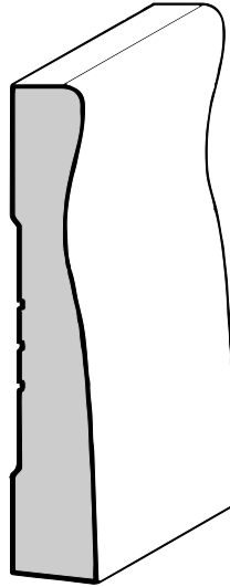
Mixon Base 9/16" X 3-1/8"
