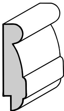
2-1/16" Colonial Cap 9/16" X 2-1/16"
