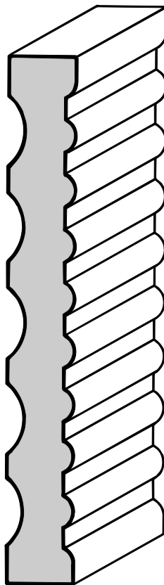
5-1/4" Beaded Casing (C-51R) 11/16" X 5-1/4"
