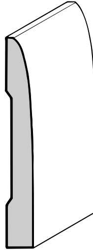
Sanitary Base 3/8" X 3", 3-1/8", 3-1/4"
