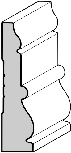
C-3011 Casing 11/16" X 2-7/8"
