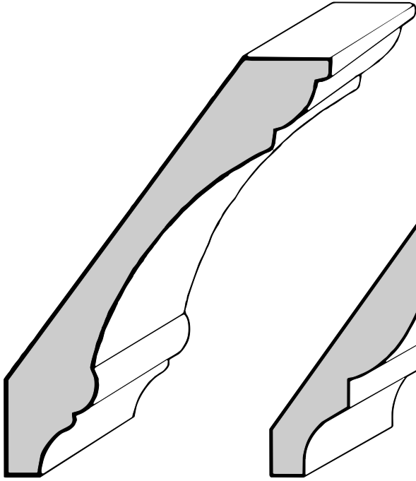
5" Cove 7/8" X 5-1/4"
