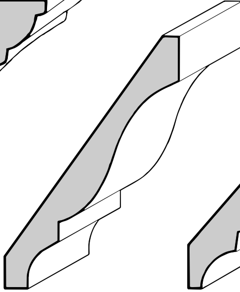
8012 Crown 9/16" X 4-1/4"
