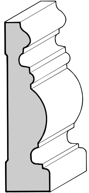
C-22 Casing 1-1/8" X 4"
